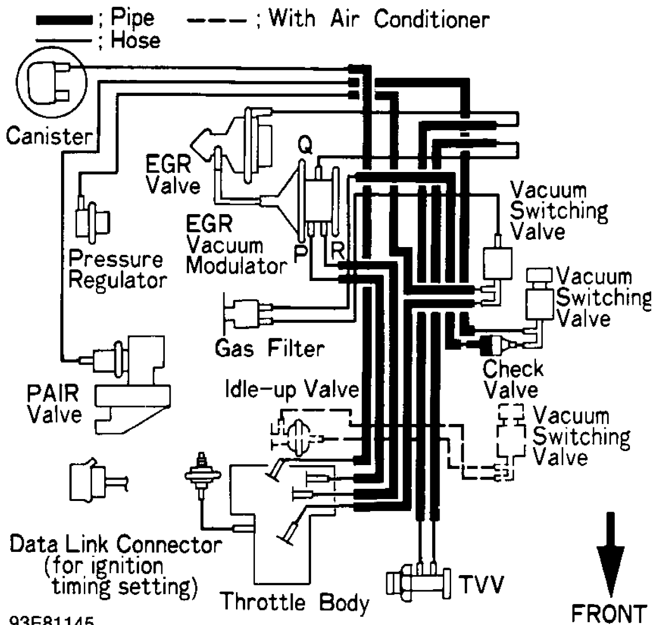
Fig. 3: Vacuum Diagram (Federal A/T) Courtesy of Toyota Motor Sales, U.S.A., Inc.
