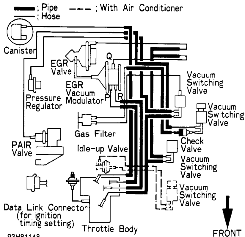
Fig. 1: Vacuum Diagram (Calif. A/T) Courtesy of Toyota Motor Sales, U.S.A., Inc.
