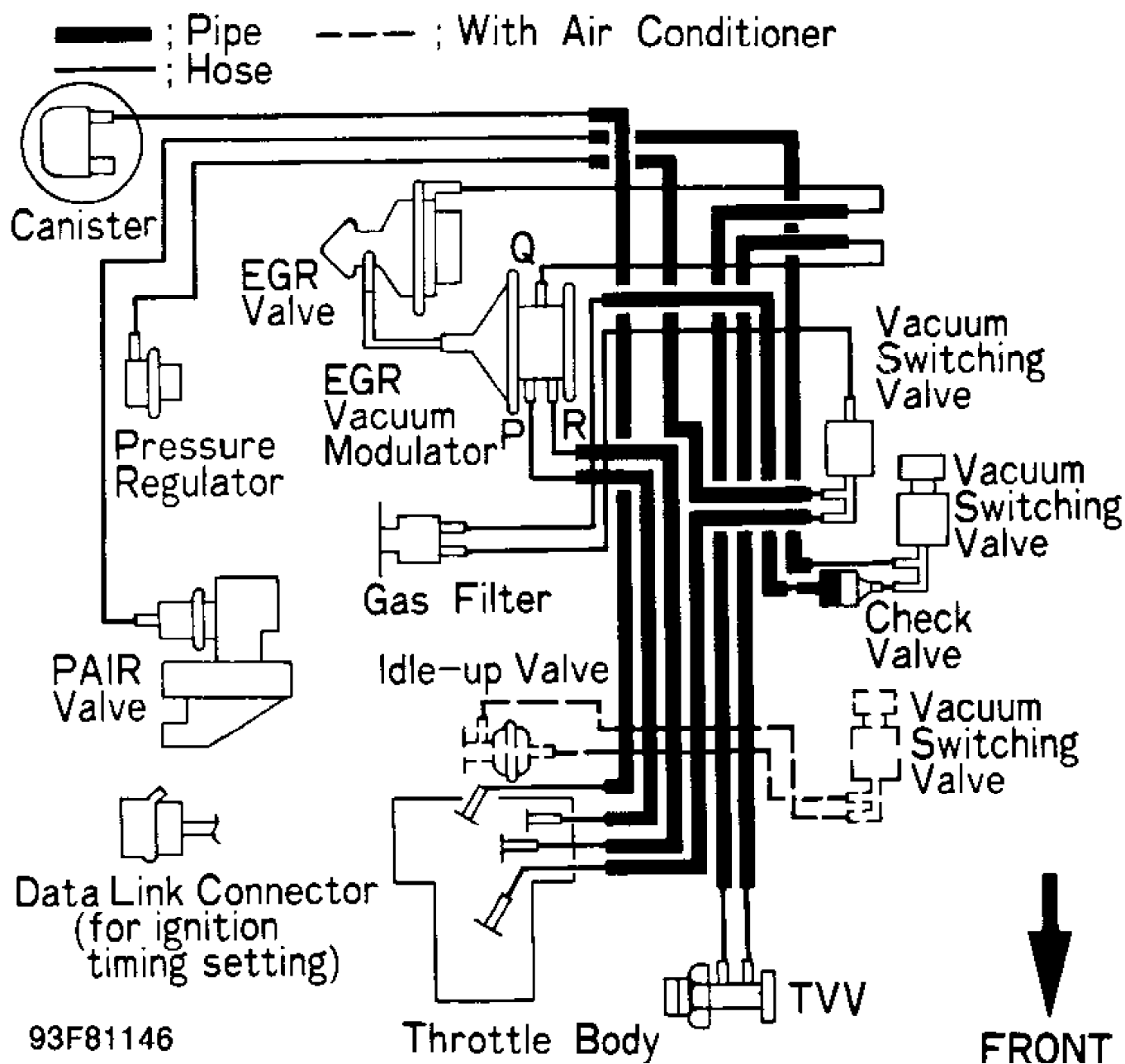
Fig. 4: Vacuum Diagram (Federal M/T) Courtesy of Toyota Motor Sales, U.S.A., Inc.
