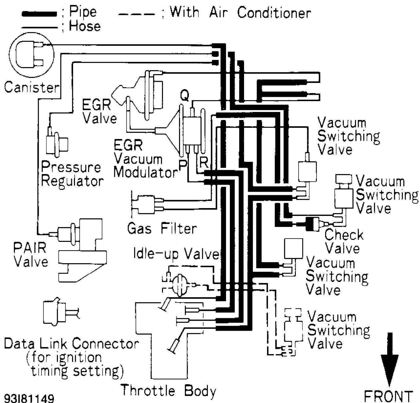
Fig. 2: Vacuum Diagram (Calif. M/T) Courtesy of Toyota Motor Sales, U.S.A., Inc.
